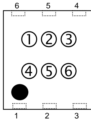
DFN(PLP)1820-6 Part Markings
